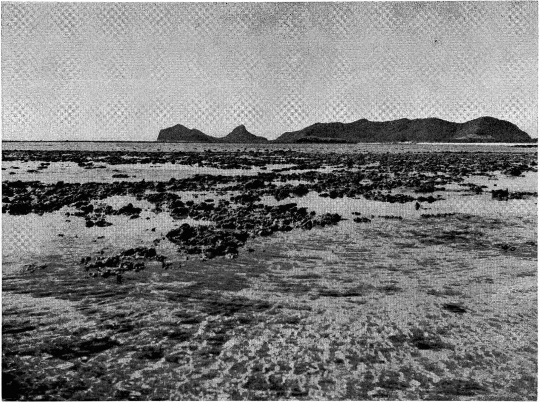
FIG. 7. The lagoon viewed from the south during low tide. In the foreground are coral reefs, of interest to the marine zoologist; behind these is low Rabbit Island, and in the background is the northern part of the island with tooth-shaped Mt. Eliza. (Photo by Miss Z. Liepa.)
